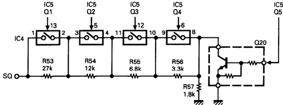
Fig. 4 Squelch circuit
