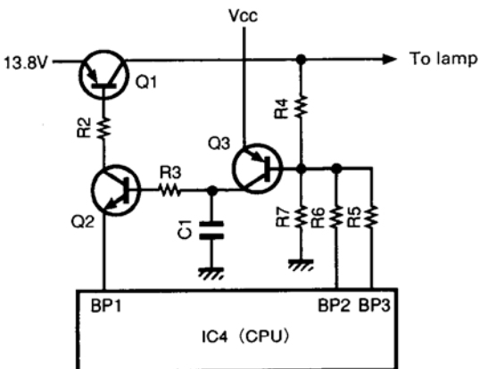
Fig. 15 Dimmer circuit
